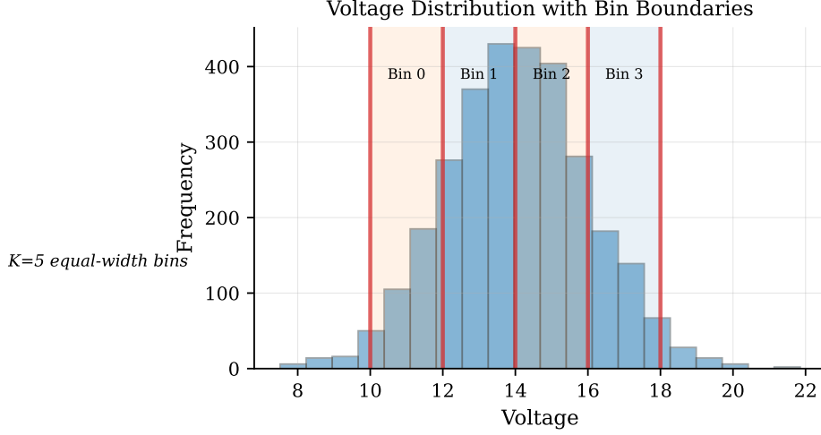
Figure 12: Feature binning: continuous values mapped to categorical bins.
