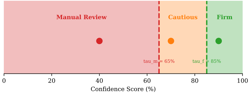
Figure 17: Confidence threshold regions mapping scores to decision categories.
