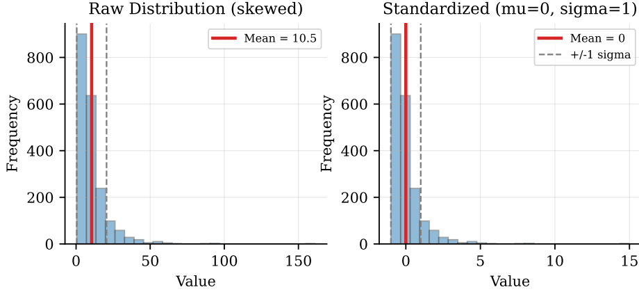
Figure 11: Effect of standardisation: raw distribution (left) vs. standardised distribution (right).
